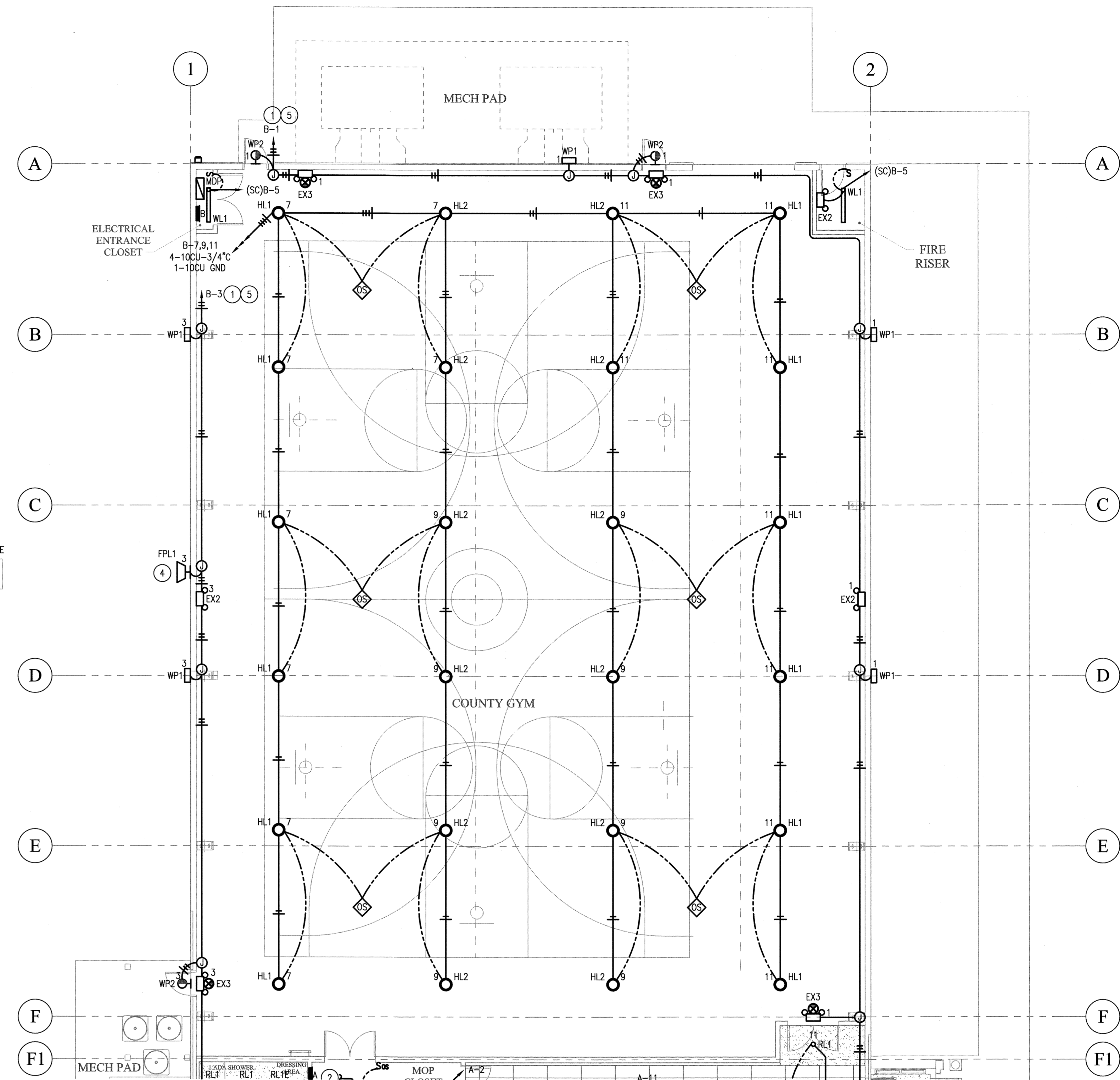
LIGHTING PLAN-GYM SCALE: 1/8"=1'-0"
