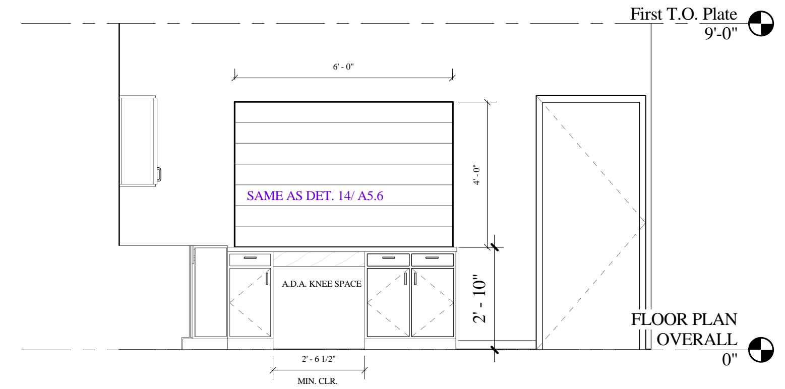
16 KITCHEN SERVE COUNTER NORTH 3/8" = 1'-0"
